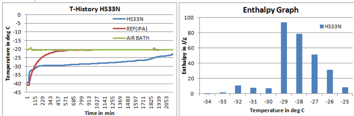
Fig1: T-History graph for HS33N done in air bath
