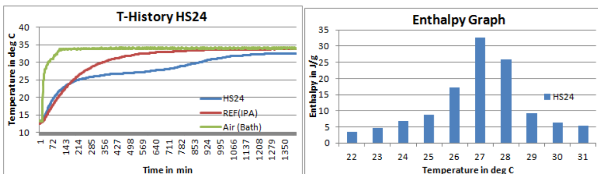
Fig1: T-History graph for HS24 done in air bath
