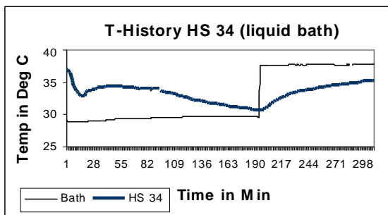
T-History graph for savE ® HS 34
