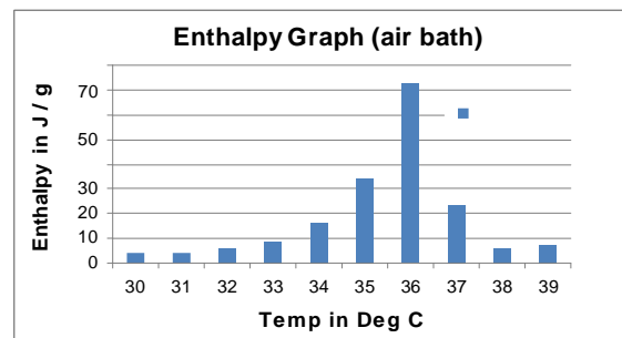
Enthalpy Vs Temp for savE ® HS 34
