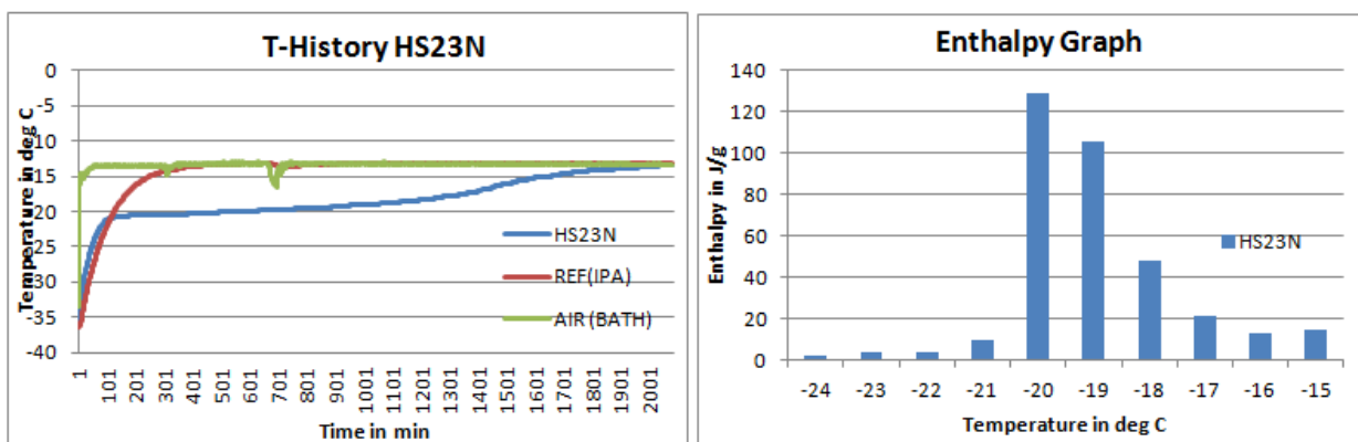
Fig1: T-History graph for HS23N done in air bath
