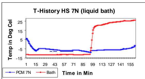
T-History graph for HS 7N
