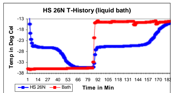
T-History graph savE ® HS 26N
