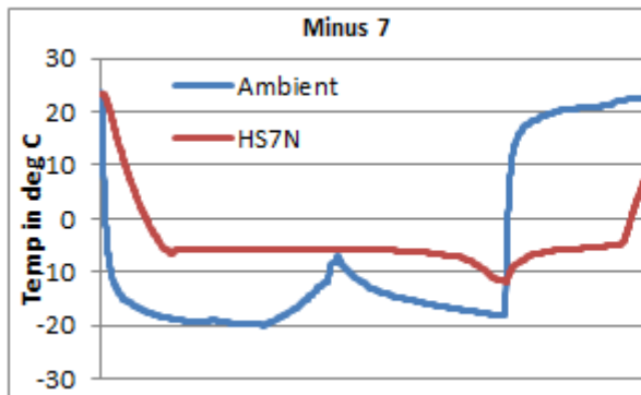
T-History graph of savE® Minus7™
