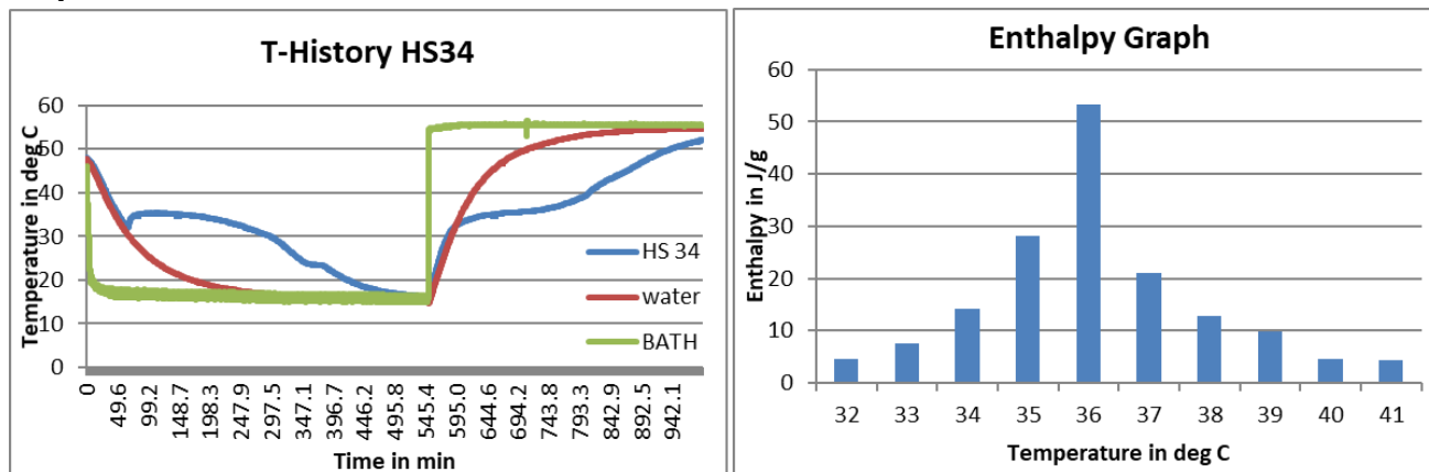
Fig1: T-History graph for HS34 done in air bath
