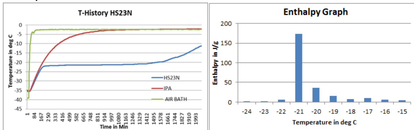
Fig1: T-History graph for HS23N done in air bath
