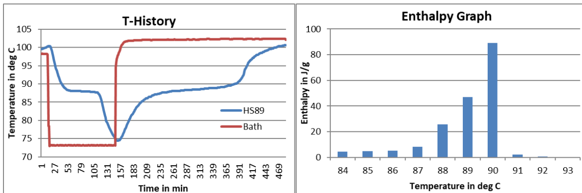
Fig1: T-History graph for HS89
