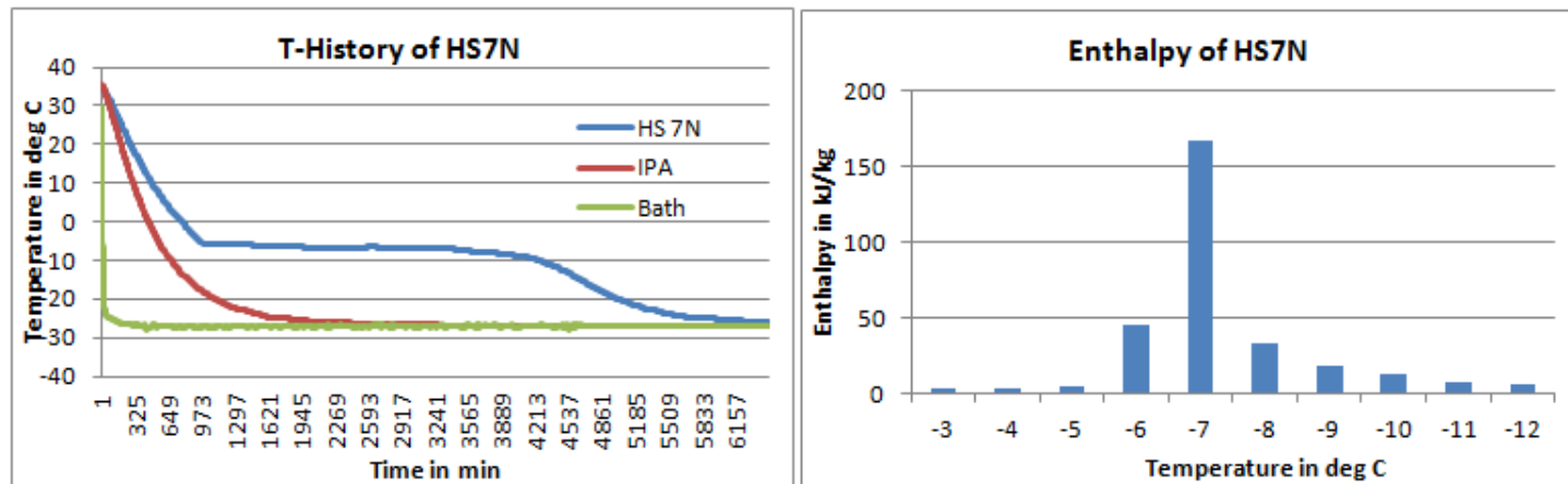
Fig 1: T-History Graph of HS7N
