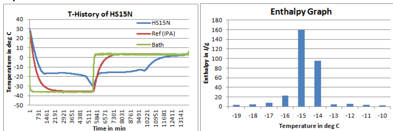
Fig1: T-History graph for HS15N done in air bath
