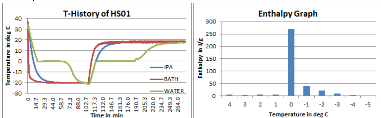
Fig 1: T-History graph of HS01 in air bath
