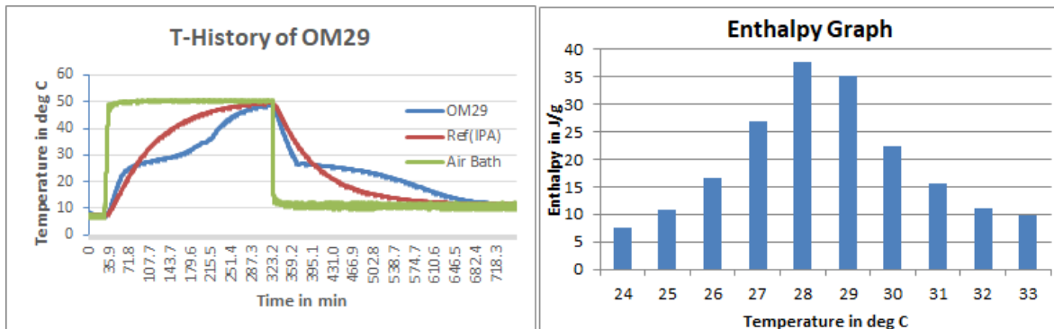
Fig1: T-History graph for OM29 done in air bath
