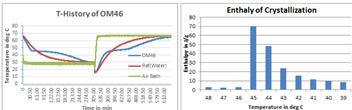
Fig 2: T-history Method of OM46
