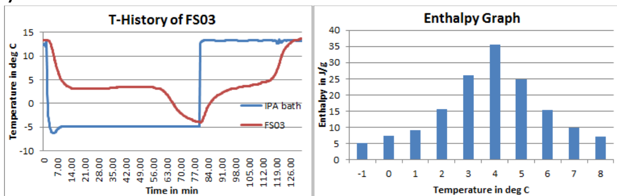
Fig1: T-History graph for FS03 done in air bath
