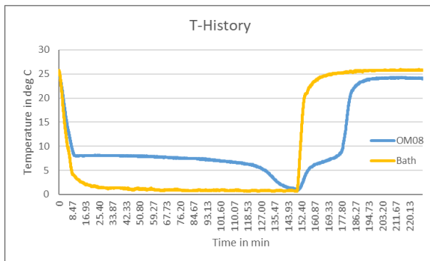
Fig1: T-History graph for OM08 done in air bath
