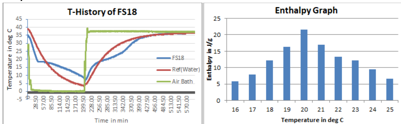
Fig1: T-History graph for FS18 done in air bath
